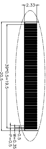
DETAIL A (4:1)
